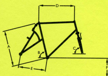
SUSPENDED MOUNTAIN BIKE GEOMETRY (Inches)
