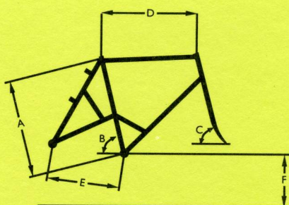
ELEVATED CHAINSTAY MOUNTAIN FRAME GEOMETRY (Inches)
