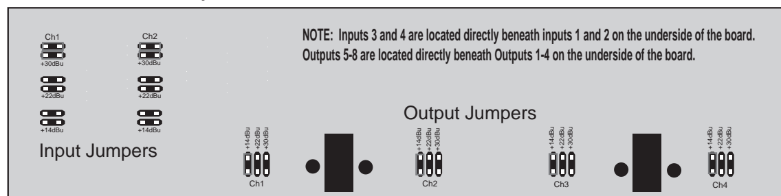
480 and 482 Top Board
