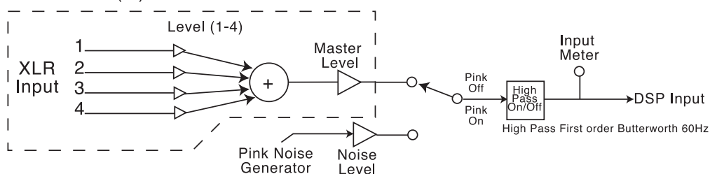
Mixer Mode (M)
