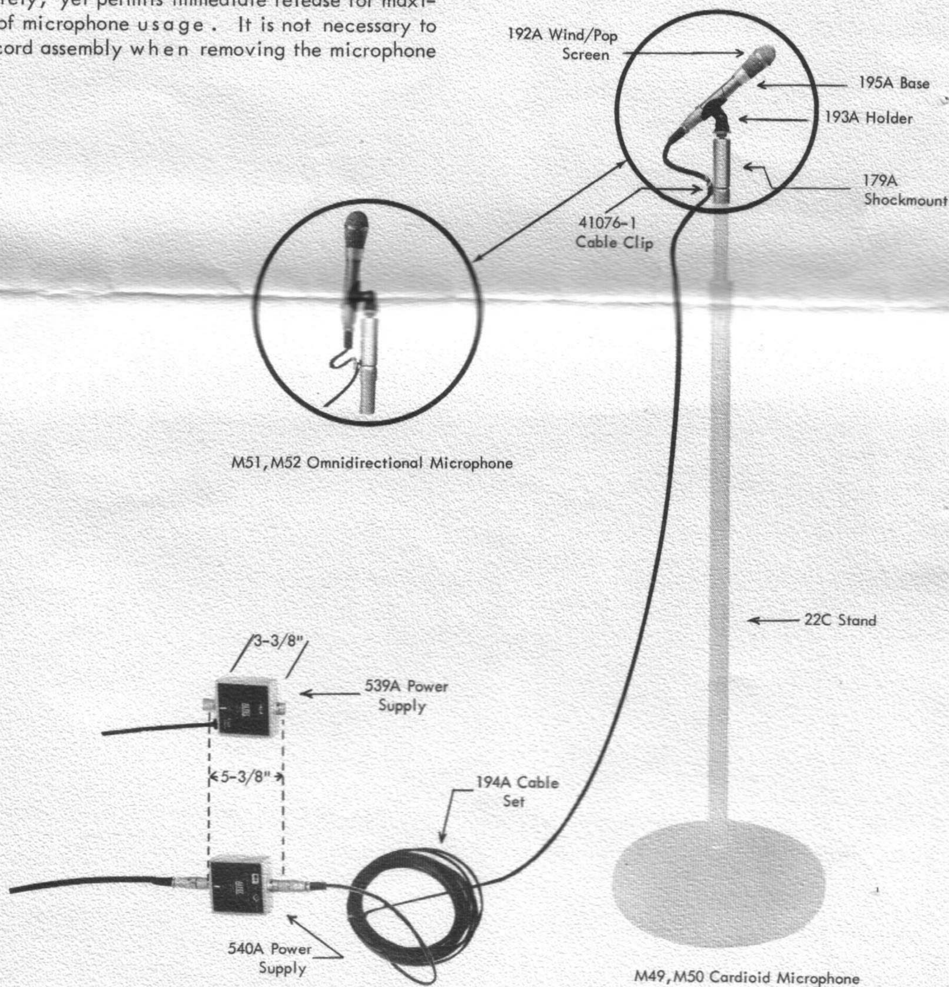
Figure 4. M49, M50, M51 and M52 Microphones
