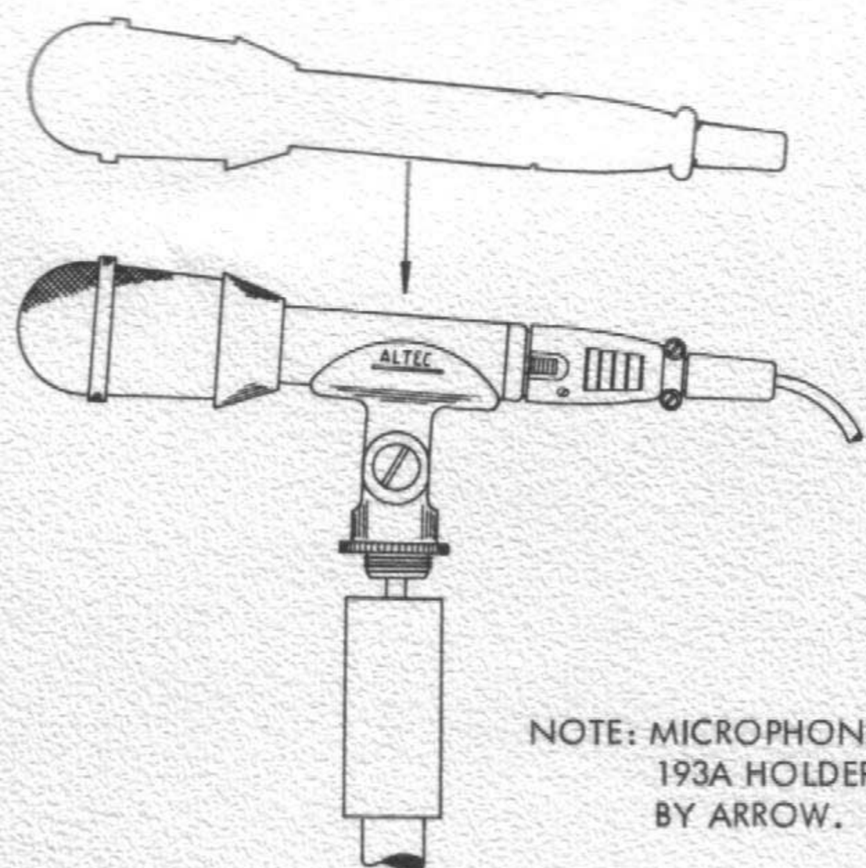
Figure 3. Snap-on Holder
