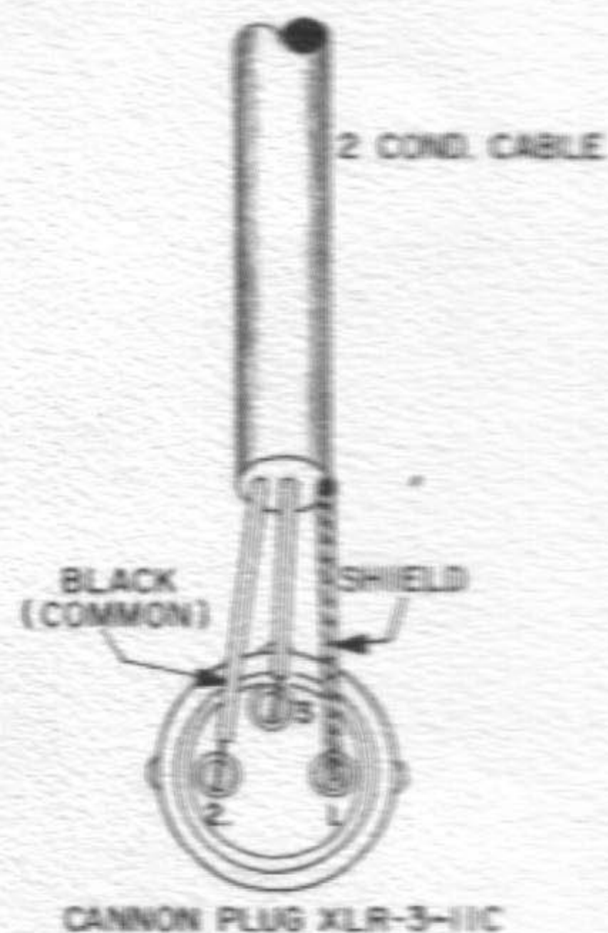
Figure 8. Microphone Cable Connection
