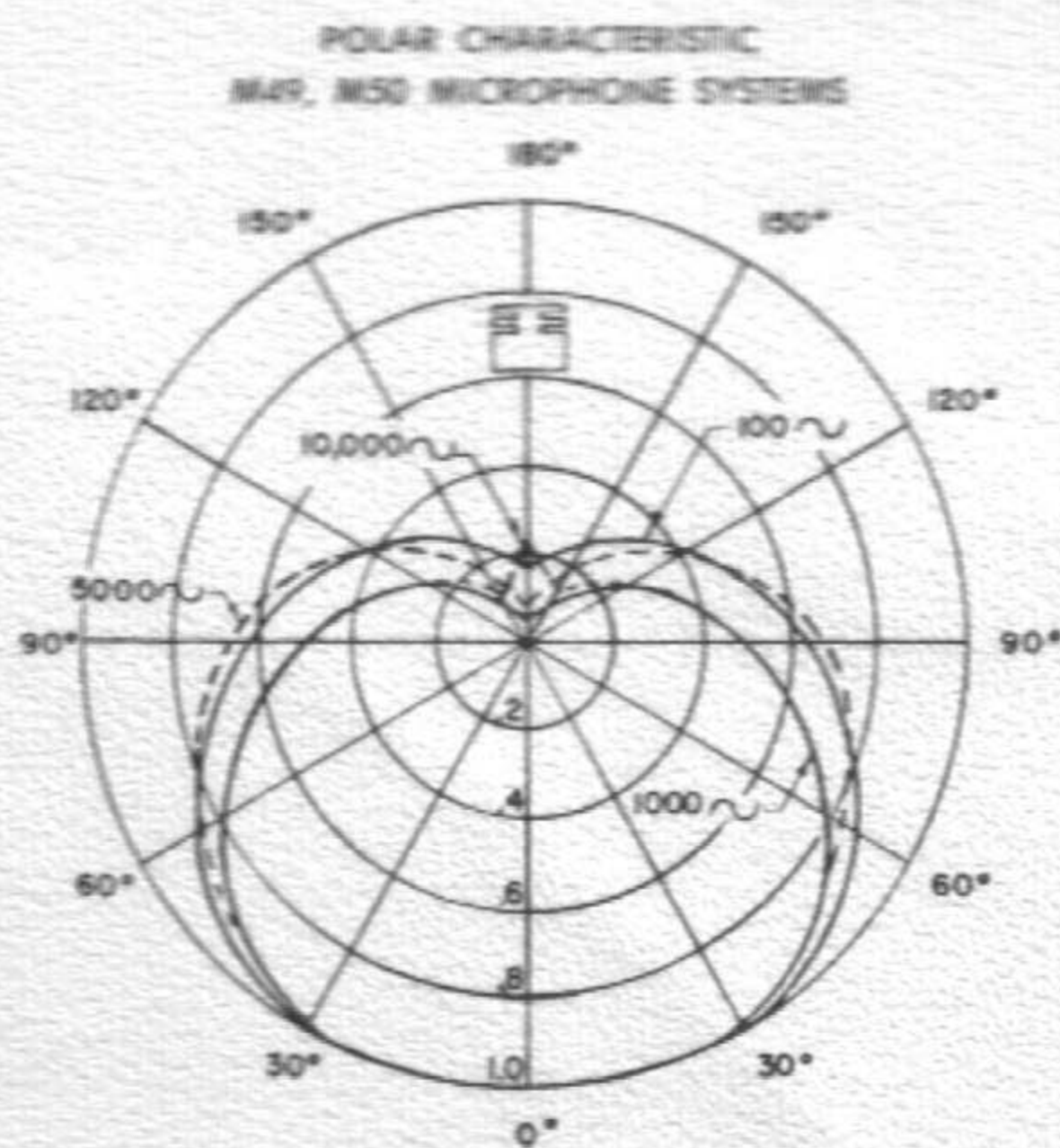
Figure 7. Polar Characteristics M49, M50 System
