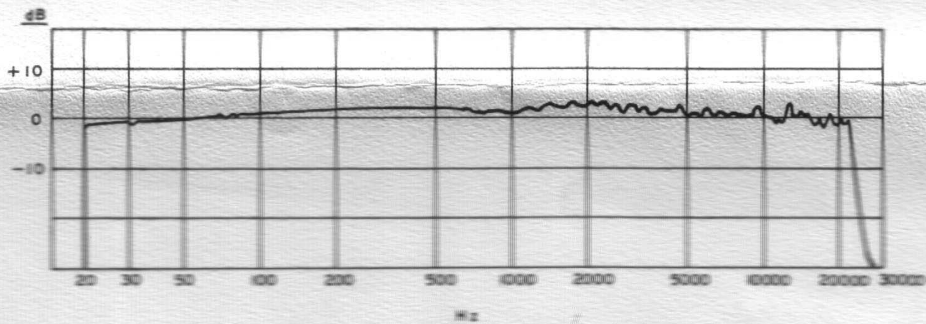
Figure 6. M51, M52 System Frequency Response
