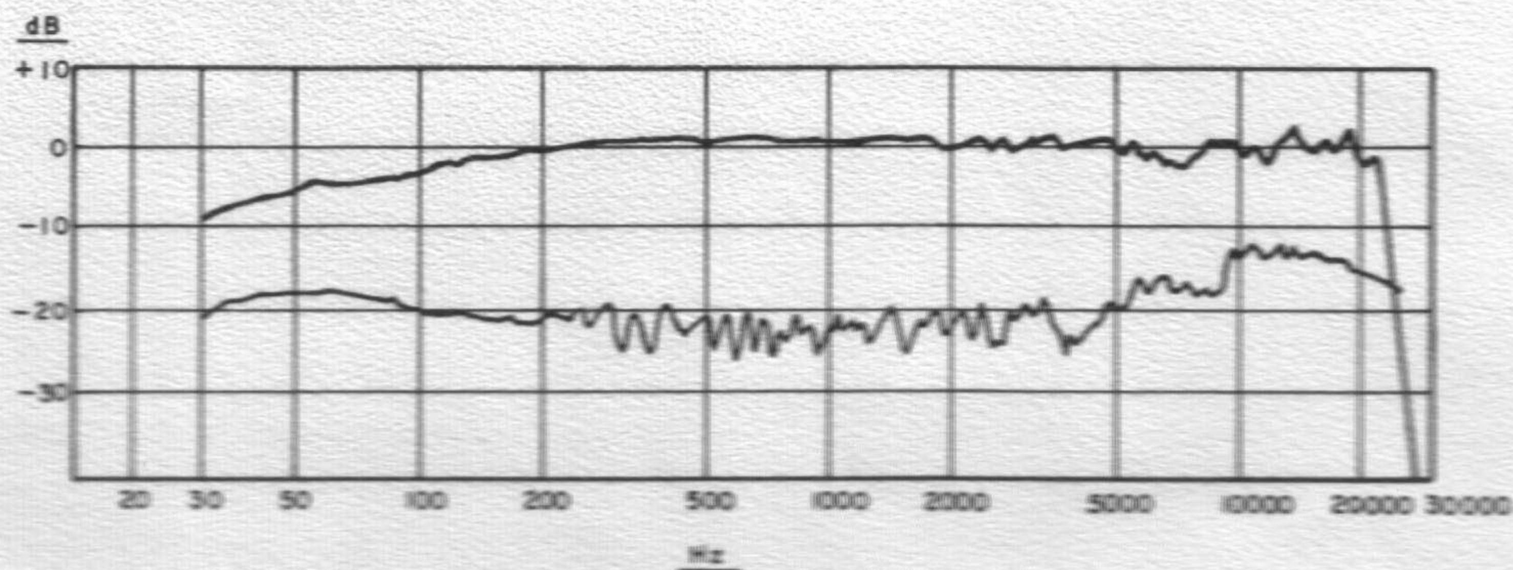
Figure 5. M49, M50 System Frequency Response (Showing Front to Back Discrimination)
